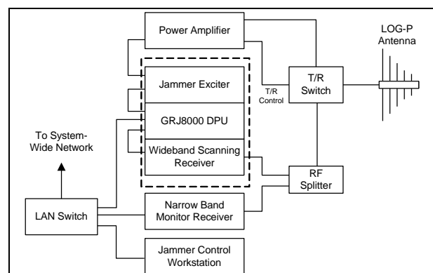
High Level System Block Diagram
