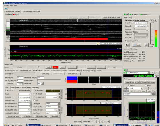
Typical user interface for Frequency Hopper signal tracking and jamming
