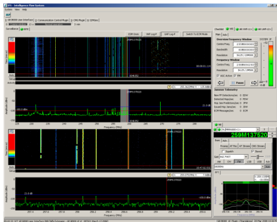
Typical spectral display for ESM functions with narrowband monitoring
