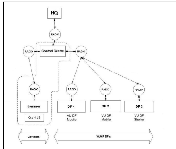
Integrated Tactical EW System
